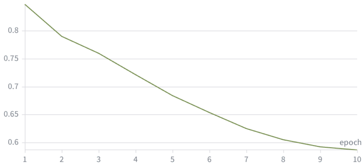
train_loss
